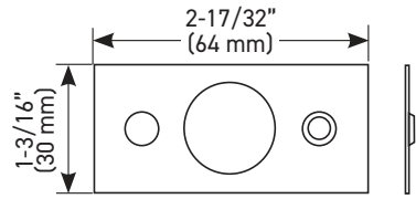
INTERIOR BRACKET
