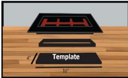
VENT COVER, RECTANGLE FRAME AND TEMPLATE
