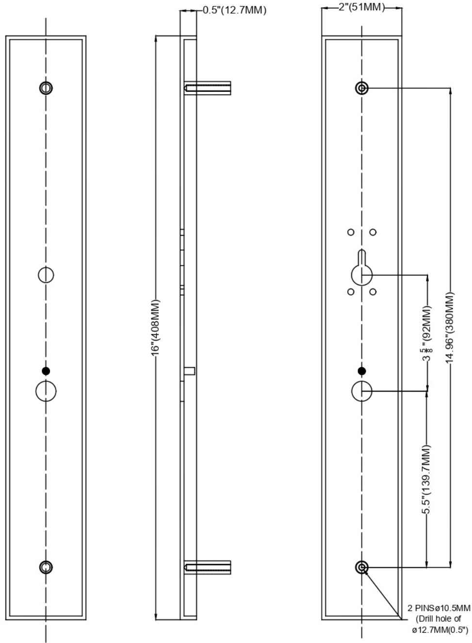
SIDE VIEW OF FRONT PLATE
